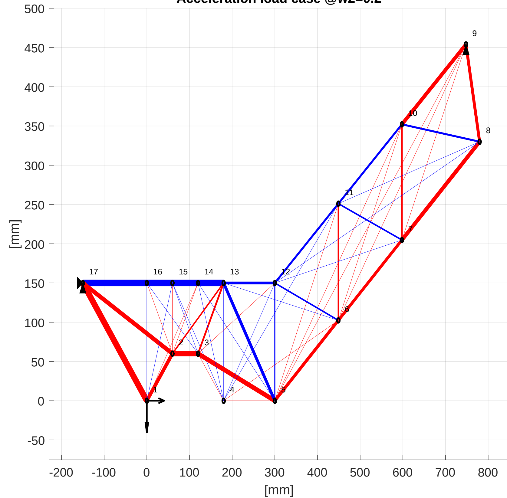
Acceleration load case @w2=0.2
