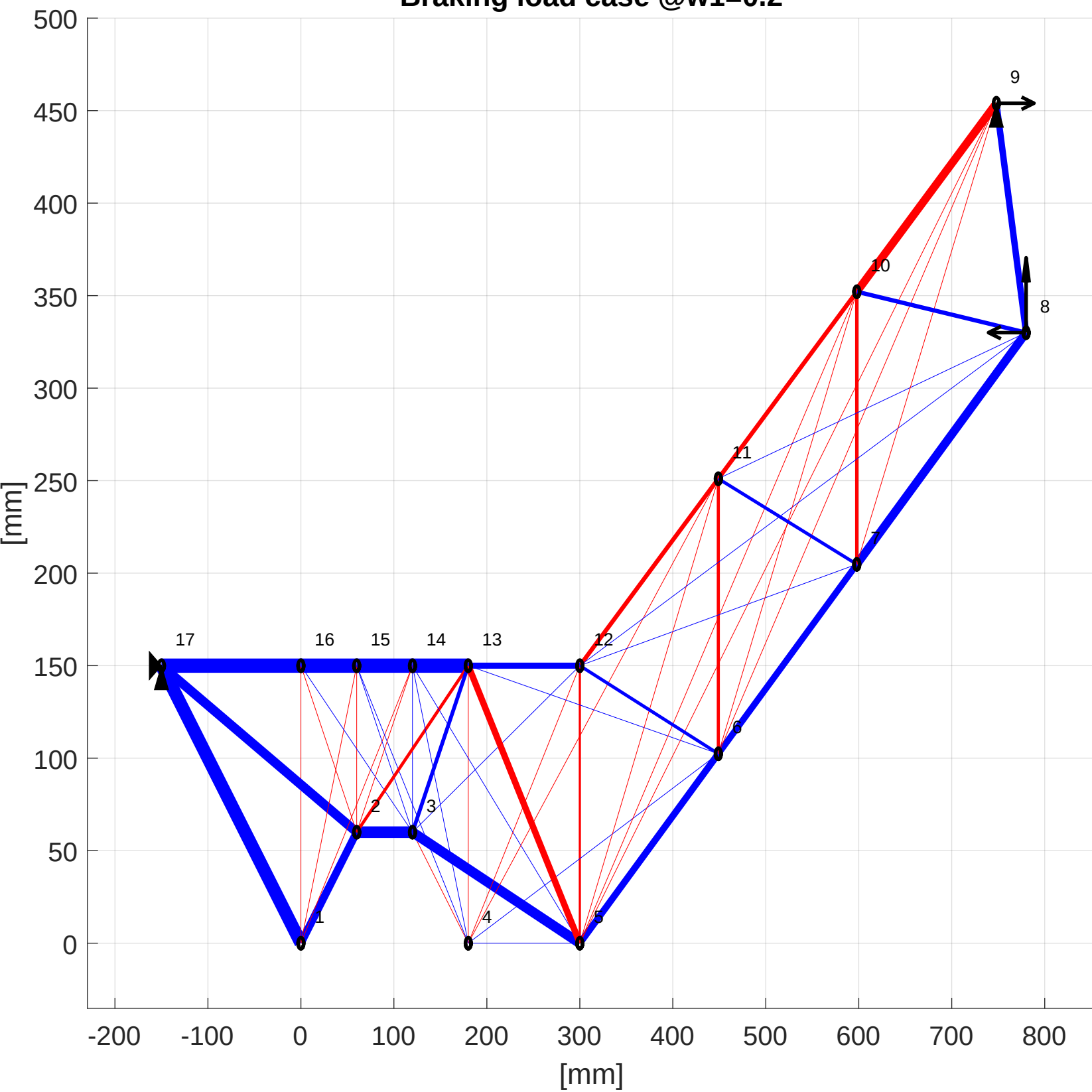
Braking load case @w1=0.2
